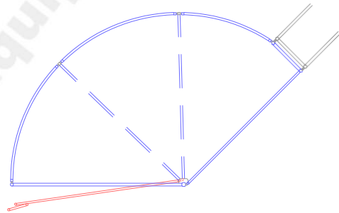
#2 LEFT AND RIGHT HAND 1/2 TUBS 10' TUBS & 12' TUBS
